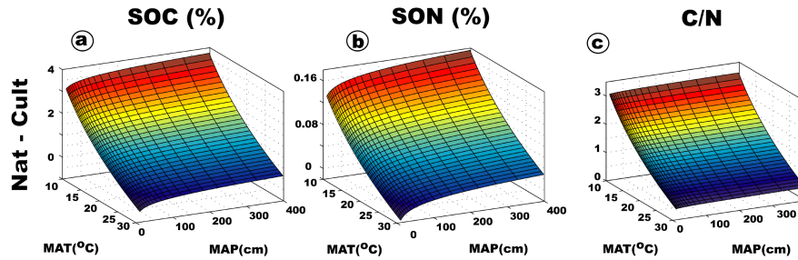
Figure 2. Multiple regression-based comparison showing absolute cultivation-induced changes in SOC, SON, and C/N as a function of climate in India
