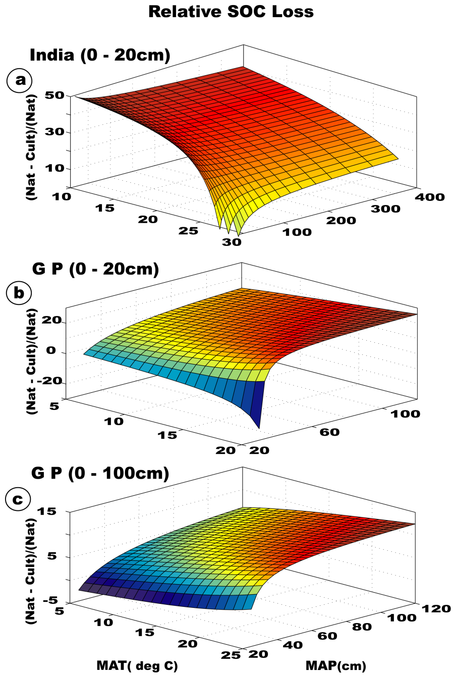
Figure 4. The relative loss in SOC from: (a) the upper 20 cm of India soils; (b) the upper 20 cm of soil in the Great Plains; (c) the upper 100 cm of soil in the Great Plains.
