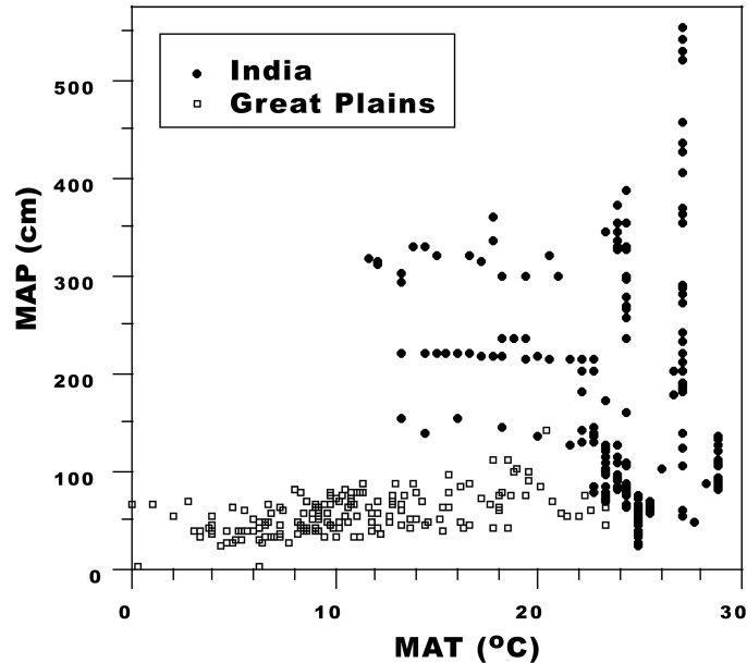
Figure 1. The climatic ranges for India and The Great Plains data sets.
