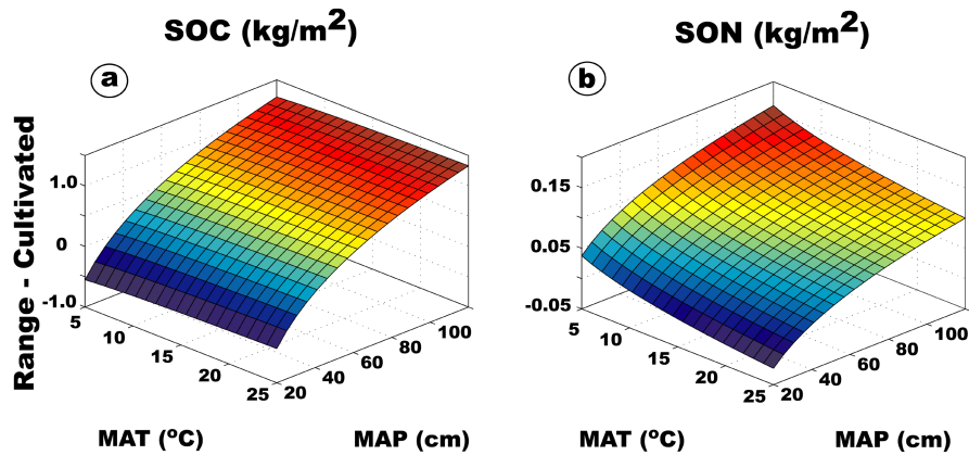
Figure 3. Multiple regression-based comparison showing cultivation-induced changes in SOC and SON as a function of climate for the Great Plains.
